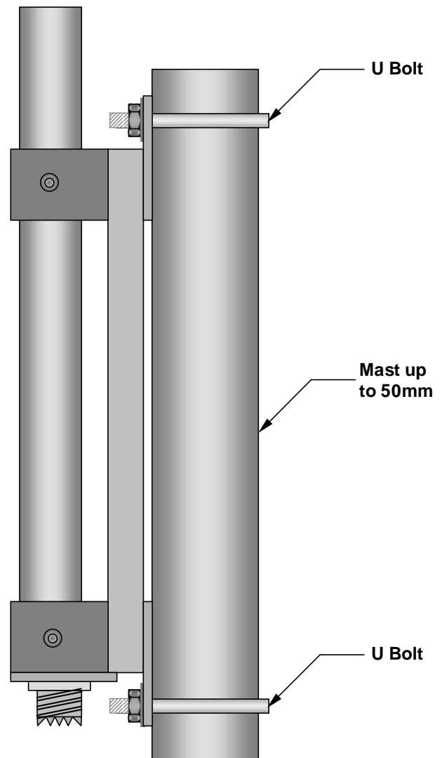
Figure 2 – Mounting Details
