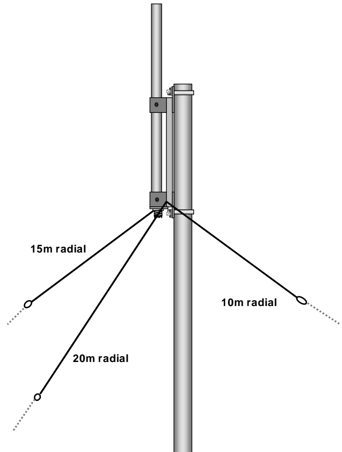
Figure 5 – Radial Installation Detail
